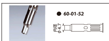
Hotblow Tip
