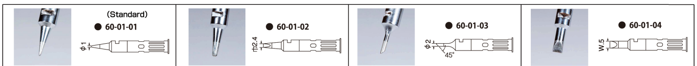
Hotblow Tip
